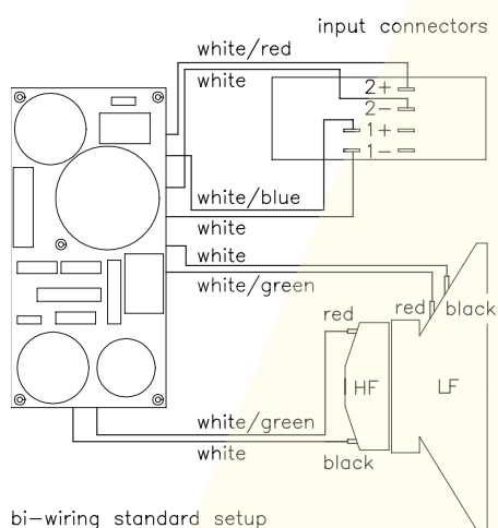
MAX wiring diagram (4-wire standard setup NL4)
