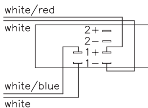
Fig. 1: MAX 2-wire operation NL4
