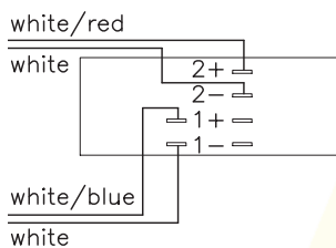
Fig. 2: MAX 4-wire operation NL4
