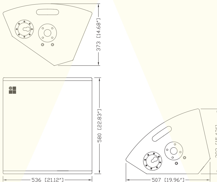
MAX cabinet dimensions in mm [inch]
